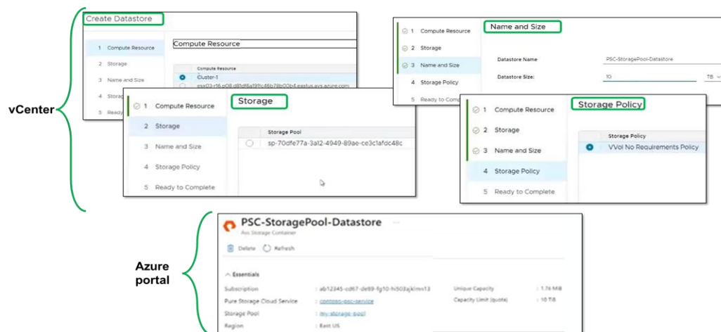
Figure 7. Using Existing VMware Tools to Create a Datastore in Microsoft Azure
