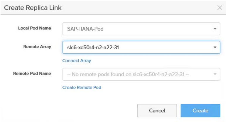
FIGURE 22 Creating the replica link.
