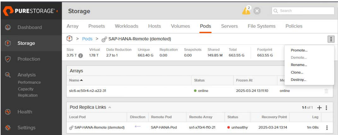
FIGURE 38 Promoting the pod on the disaster recovery array.
