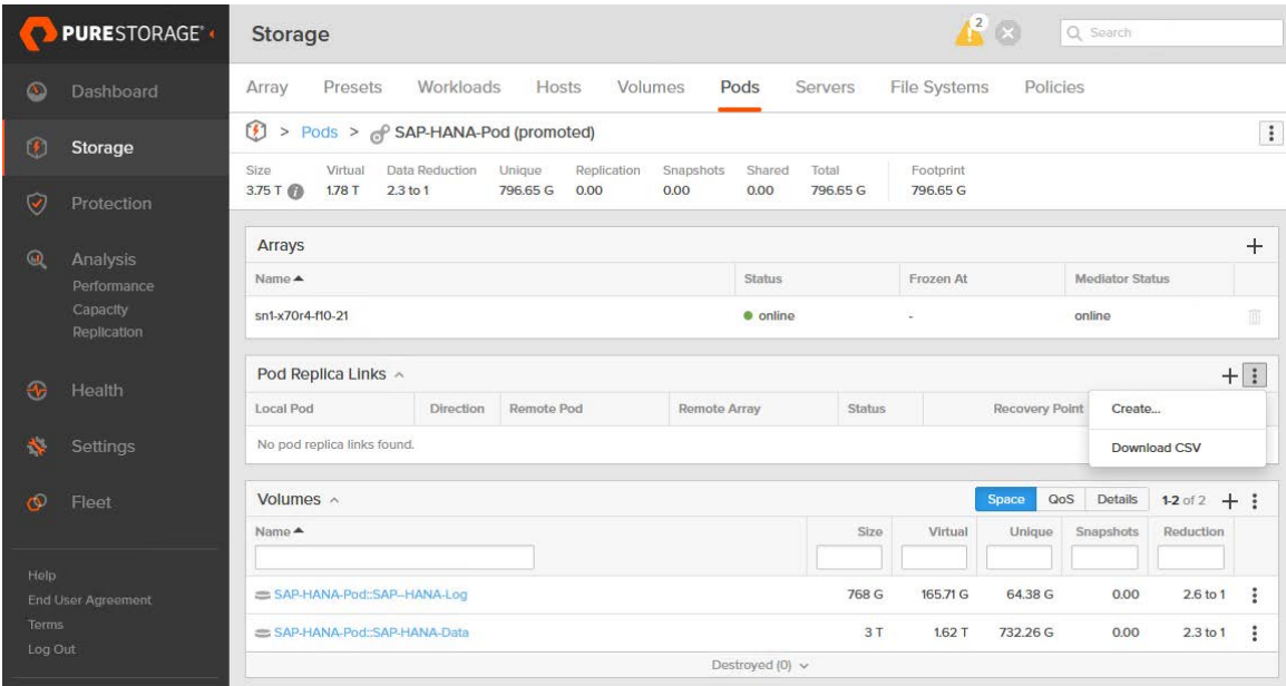
FIGURE 21 Creating a replica link for the previously created pod.
