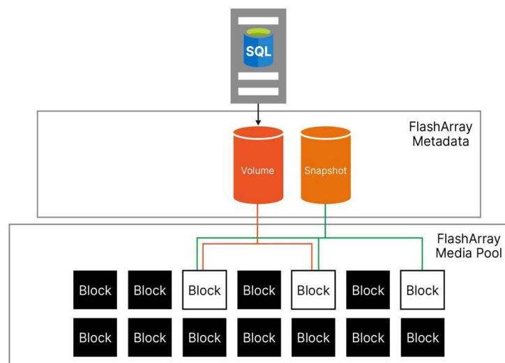
FIGURE 2 FlashArray volumes and snapshots use metadata pointers to reference data blocks on the FlashArray.
