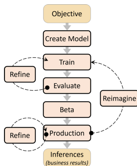
FIGURE 1 AI Project Life Cycle
