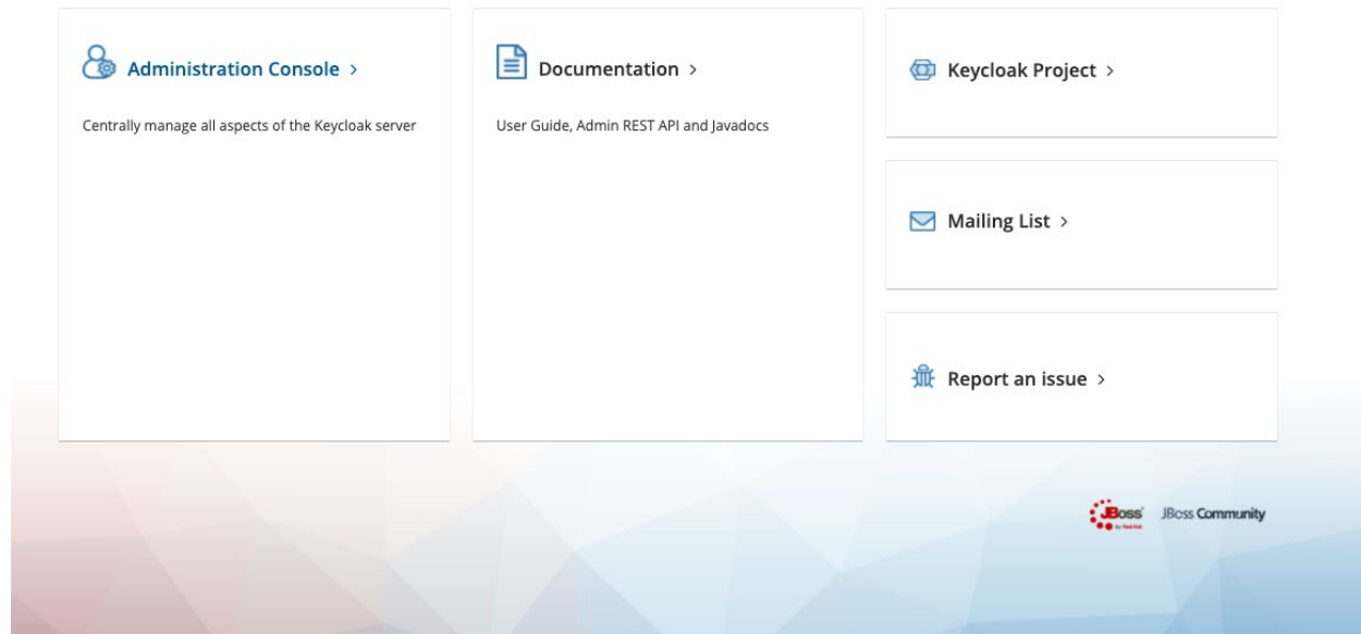
Figure 38: Keycloak interface
