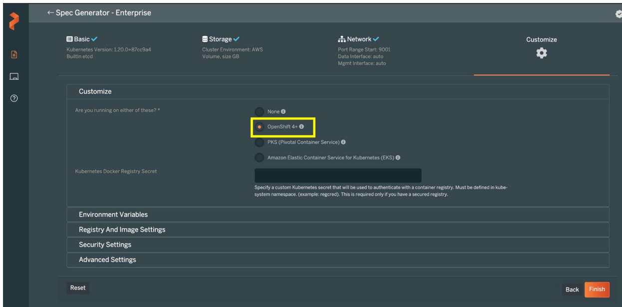
Figure 7. Customizing OpenShift 4+
