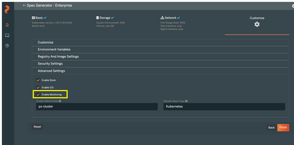
Figure 11: Enabling monitoring
