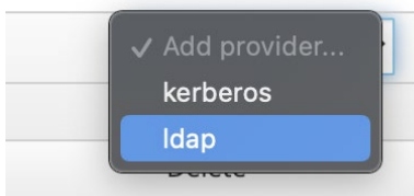
Figure 40: Adding Idap
