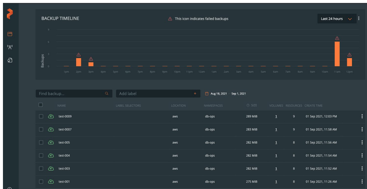
Figure 51: Backup timeline
