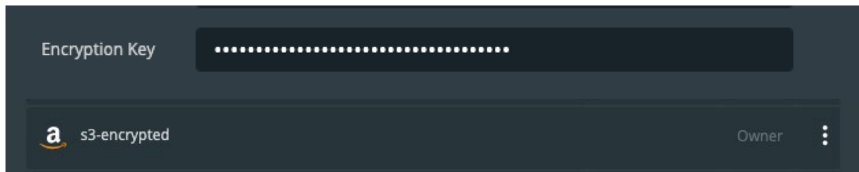
Figure 66: Encryption key
