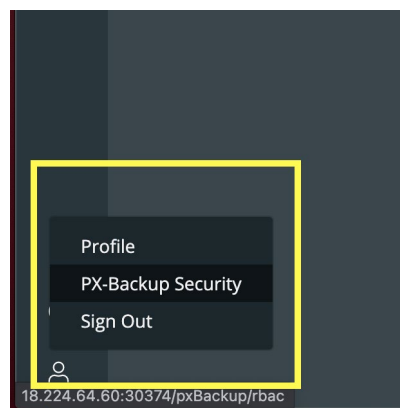
Figure 37: PX-Backup Security
