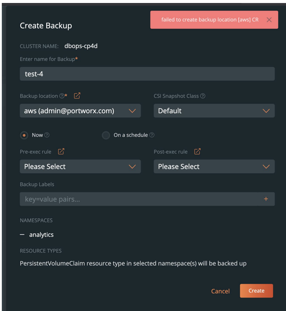
Figure 55: Backup error
