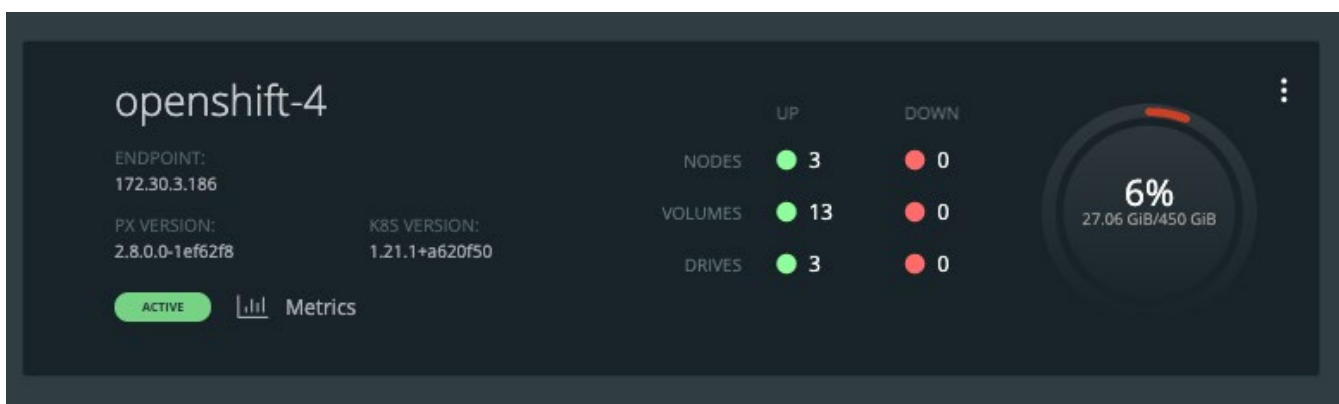
Figure 19: Monitoring dashboard
