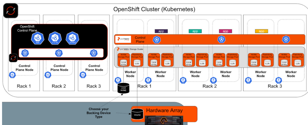
FIGURE 1 General reference architecture
