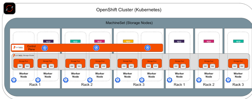
FIGURE 4 Hyper-converged architecture
