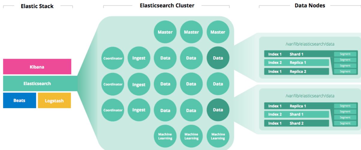
Figure 6: Elasticsearch Architecture
